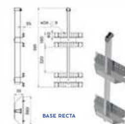
BASE RECTA
